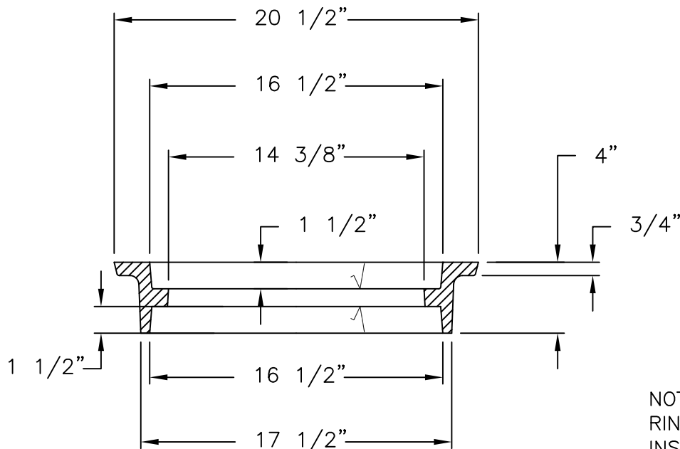
RING SECTION
